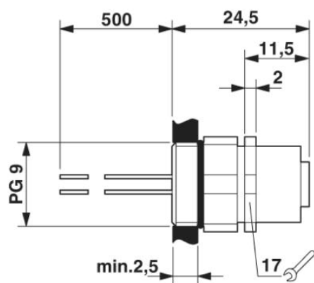
M12-inbouwconnector
