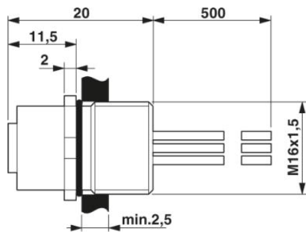
M12-inbouwconnector
