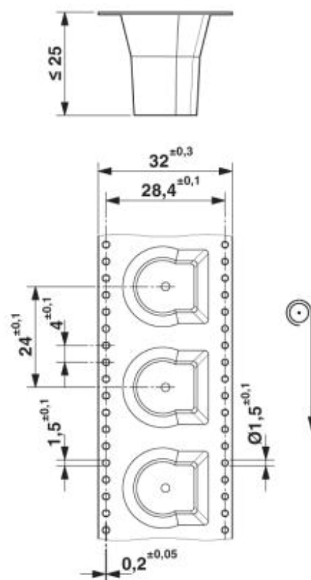
THR-rolverpakking (Tape-on-Reel)
