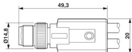
Stiftconnector M12 x 1, Y-verdeler
