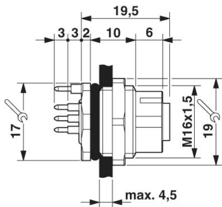
M12-inbouwconnector
