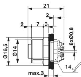
M12-inbouwconnector
