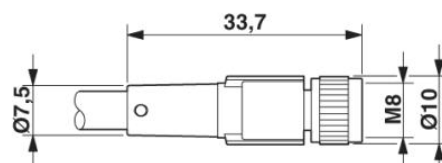
Bus M8 x 1, recht
