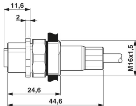
M12-inbouwconnector
