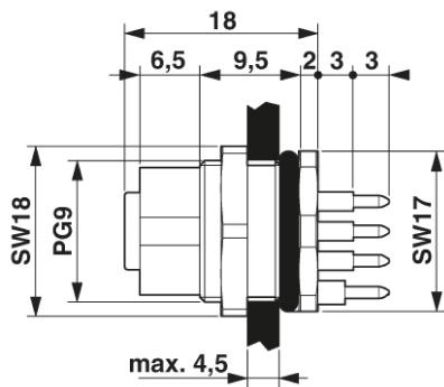
M12-inbouwconnector
