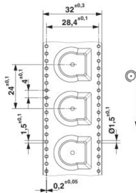
THR-rolverpakking (Tape-on-Reel)
