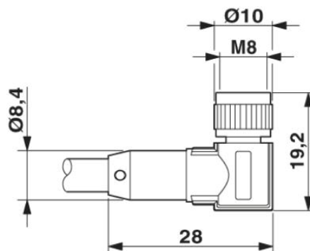
Bus M8 x 1, haaks, met led
