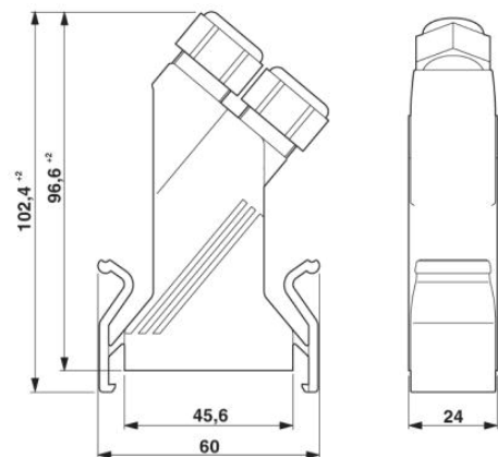
D-SUB-wartelbehuizing
