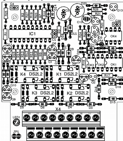
Fig.1 : Printplan (SD-34)
