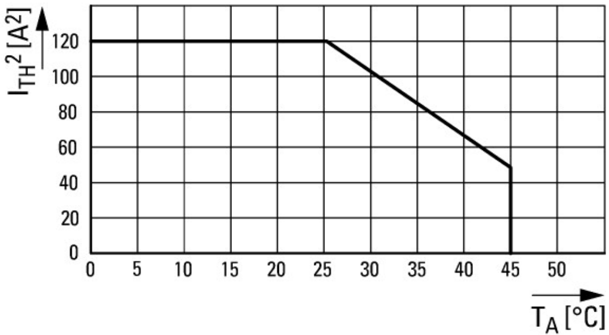
Derating-curve
