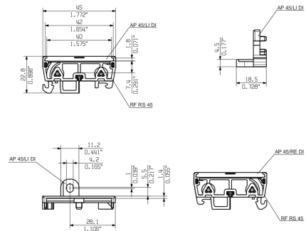
DIRECT MOUNTING
