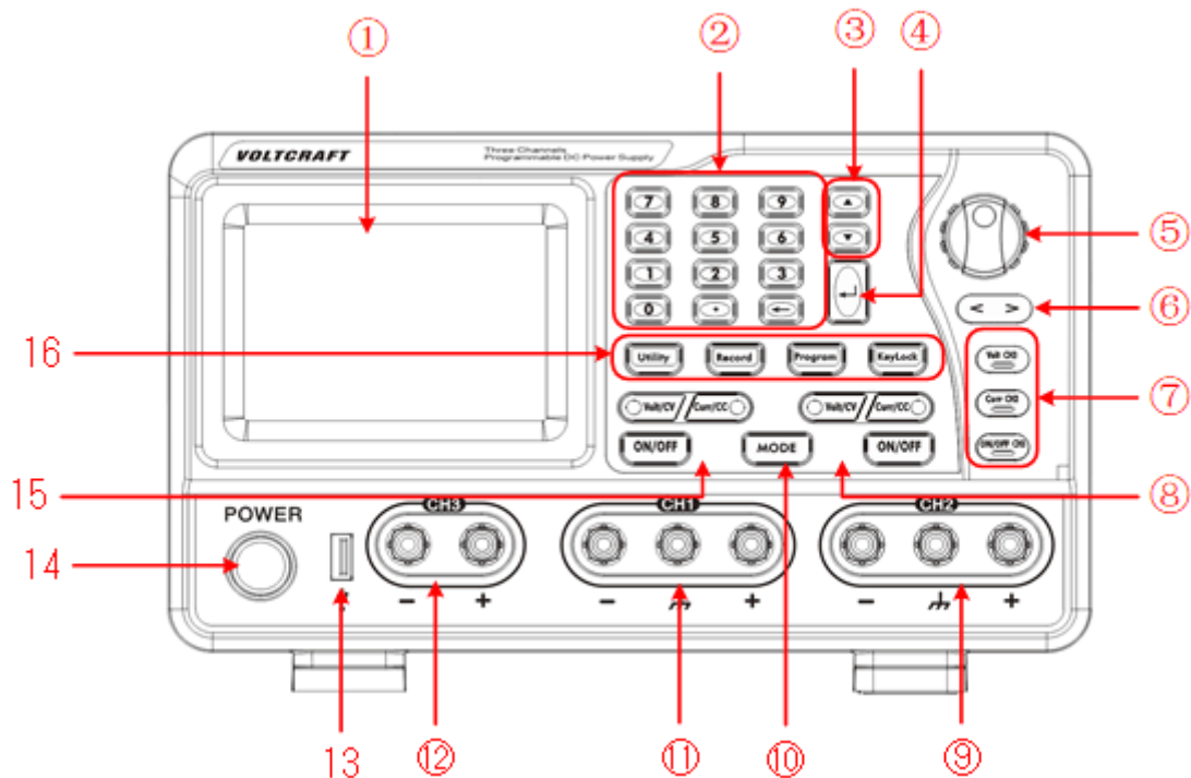
Figure 3-1 Front panel overview
