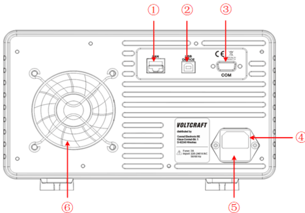
Figure 3-2 Rear panel overview
