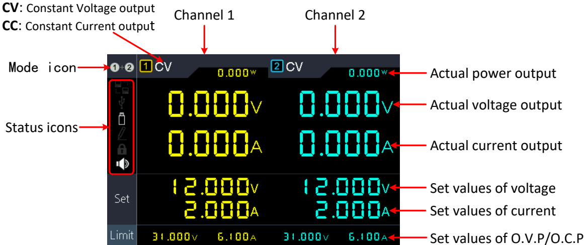
Figure 3-4 User interface in Dual channel mode
