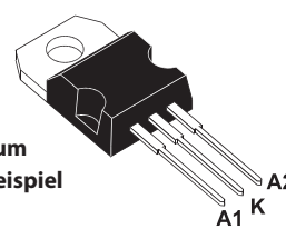
TO-220AB STPS30L40CT
